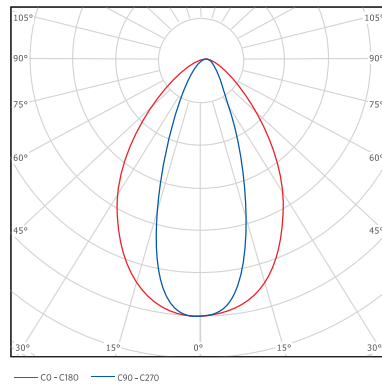
72°+28° (150W/200W)
