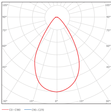
60° (150W/200W)
